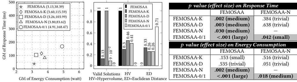
Fig. 21. Results with MOEA/D-STM under read-write pattern on RUBiS-SAS. (GM denotes Geometric Mean. The significant statistics of comparisons, i.e., p < 0.05 , are highlighted and shown in bold.)
