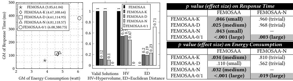
Fig. 22. Results with NSGA-II under read-write pattern on RUBiS-SAS. (GM denotes Geometric Mean. The significant statistics of comparisons, i.e., p < 0.05 , are highlighted and shown in bold.)
