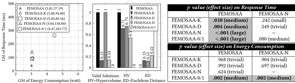
Fig. 25. Results with NSGA-II HV under read-only pattern on RUBiS-SAS. (GM denotes Geometric Mean. The significant statistics of comparisons, i.e., p < 0.05 , are highlighted and shown in bold.)
