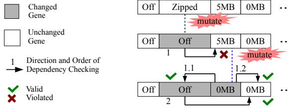
Fig. 16. Workflow of dependency aware mutation operator. (The example genes from left to right represent Transmission Compression , Cache Mode , Heap Size and Disk Size )
