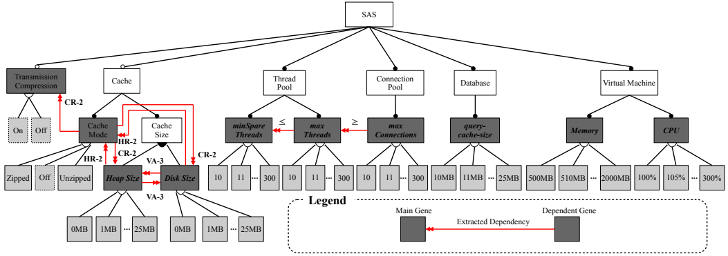
Fig. 12. The example SAS's feature model and the extracted dependency after the process of VA, HR and CR.
