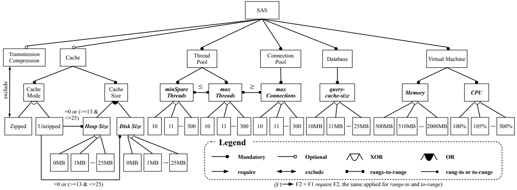
Fig. 4. The feature model for the example SAS shown in Figure 1. (The numeric features are shown in bold and italic letters. A zipped cache mode means the cached data is compressed, thereby costing smaller amount of memory; otherwise, it is unzipped. CPU % denotes to what extent the SAS can consume CPU capacity where each 100% means a CPU core, e.g., 200% means two cores; 150% means one full core and 50% of another)
