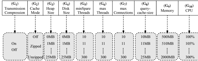
Fig. 8. The resulted chromosome representation of the SAS studied in form of genes ( G_1, G_2, \dots, G_{10} ).
