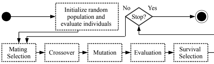
Fig. 2. The general workflow of MOEA.
