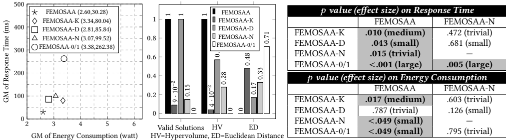
Fig. 24. Results with MOEA/D-STM under read-only pattern on RUBiS-SAS. (GM denotes Geometric Mean. The significant statistics of comparisons, i.e., p < 0.05 , are highlighted and shown in bold.)
