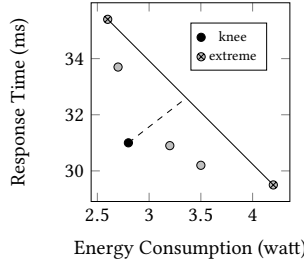
Fig. 18. Finding knee solution(s) in the non-dominated set.
