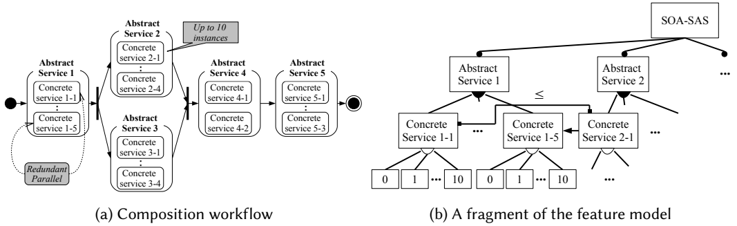
Fig. 20. The architecture of SOA-SAS.
