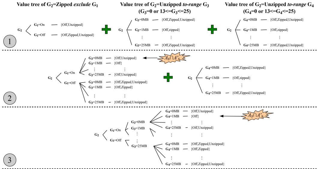
Fig. 14. The example of dependency merging and the combined value tree for the gene G_2 (Cache Mode), which is the dependent gene of three different main genes, i.e., G_1 (Transmission Compression), G_3 (Heap Size) and G_4 (Disk Size). A_s and A'_s denote two sets of values (leaf-set) to be combined, as specified in Table 1.
